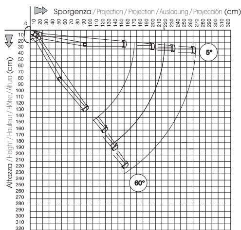
Montaggio a parete / Wall installation
